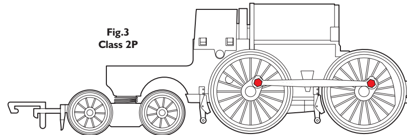
Fig.2/3 Apply one drop of oil to each of the valve gear and connecting rod pivot points indicated in red in Fig.2 and Fig.3, on both sides of the locomotive.
